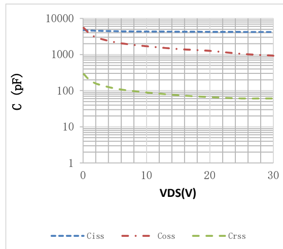
Fig.2 Capacitance Characteristics
